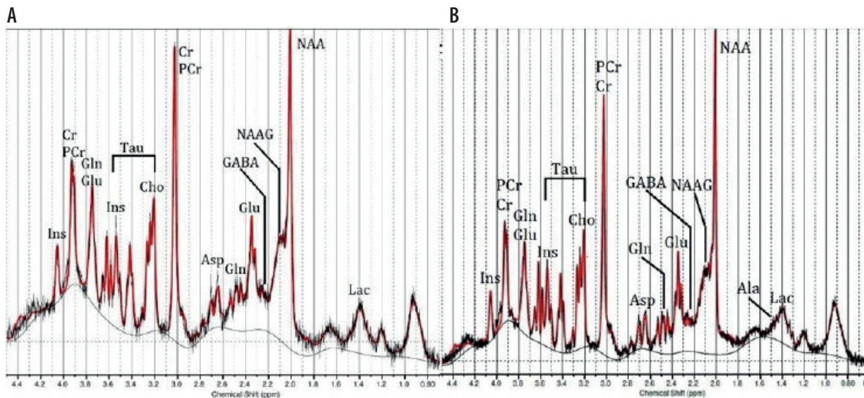
Figure 3. 1 H MRS spectra obtained at 7T. A) Spectrum from rat hippocampus, PRESS sequence: TE 16 ms, TR 2500 ms, VOI size 2 \times 2 \times 5.5 \text{ mm}^3 . B) Spectra from human white matter, PRESS, TE 17 ms, TR 2500 ms, VOI size 2 \times 2 \times 2 \text{ cm}^3 . Chemical shifts are presented relative to TMS (tetramethylsilane), ppm value on the horizontal axis in the spectra increases from right (0 ppm) to left (4.2 ppm). The window of this spectra analysis in the LCModel package was from 0.2 to 4.6 ppm. The water signal has a chemical shift value at 4.7 ppm; therefore, the water is out of range in this fitting process
